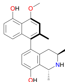
Dioncophylline C (35)
