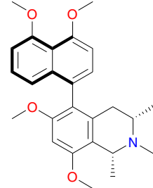
Ancistrobertsonine C (23)
