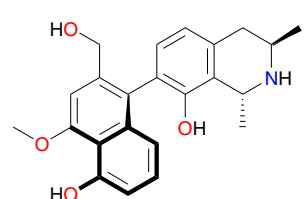
Dioncopeltine A (36)
