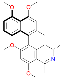
O-methylancistrocladinine (26)
