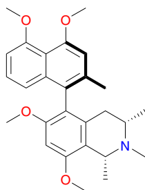
Ancistrobertsonine B (22)
