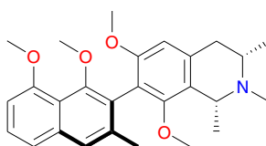
Ancistrobertsonine A (21)
