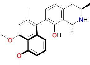
Dioncophylline A (33)
