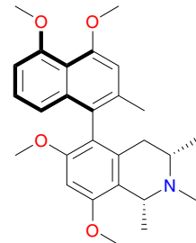
5,1'-O,N-dimethylancistrocladinine (27)
