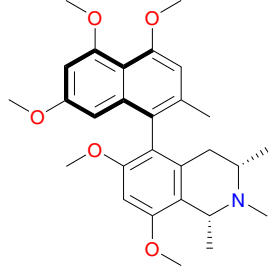
Ancistrobertsonine A (21)
