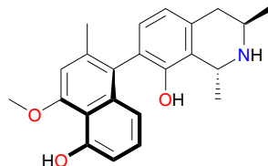
5'-O-Demethyl-dioncophylline A (31)
