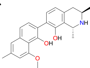
Dioncophylline B (34)
