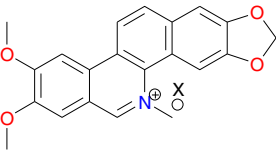
Nitidine (39)
