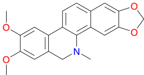
5,6-Dihydroneitidine (40)
