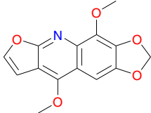
Flindersiamine (37)
