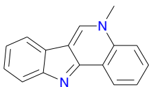
Isocryptolepine (59)
