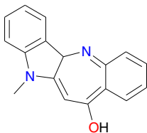
Cryptoheptine (57)
