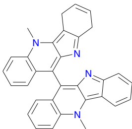
Biscryptolepine (60)
