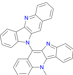
Cryptoquindoline (58)
