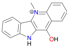
Hydroxycryptolepine (56)
