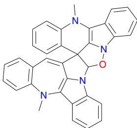
Cryptospirolepine (55)
