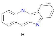
Cryptolepinoic acid (62): R = COOH
