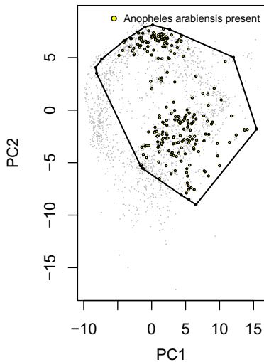
Principal Components Analysis
