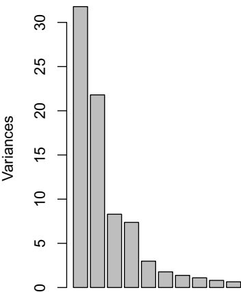
Scree plot
