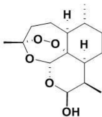
Dihydroartemisinin
