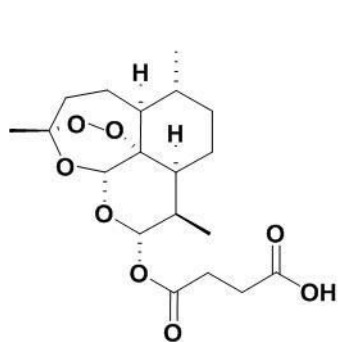
Artesunate
