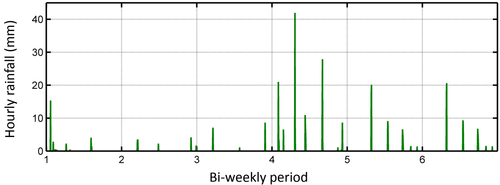
Predicted Rainfall (Pattern 2)
