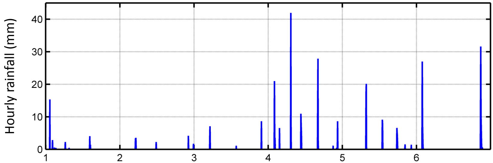
Observed Rainfall (Pattern 1)
