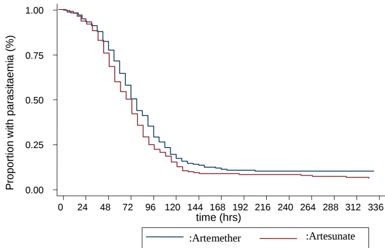
Kaplan-Meier remaining parasitaemic estimates
