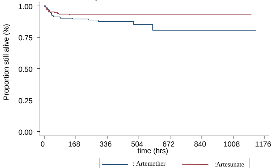
Kaplan-Meier survival estimates
