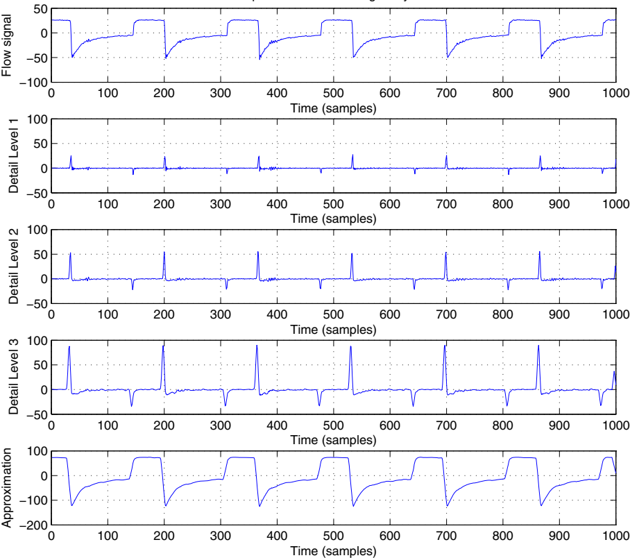
Decomposition of the flow signal by wavelet
