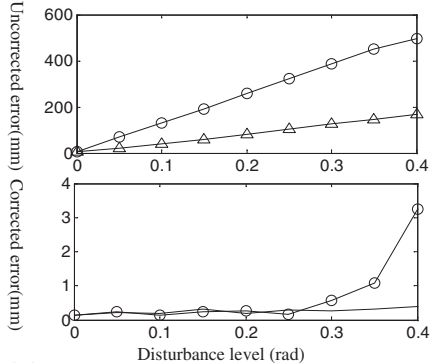
(b) ○ Joints offset resulted translational error ▲ R-T rotational error resulted translational error
