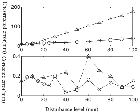
(d) ○ Link length error resulted translational error ▲ R-T translational error resulted translational error
