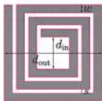
(a) Square Coil
