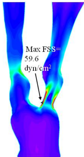
(c) FSS, Bifurcation Cut
