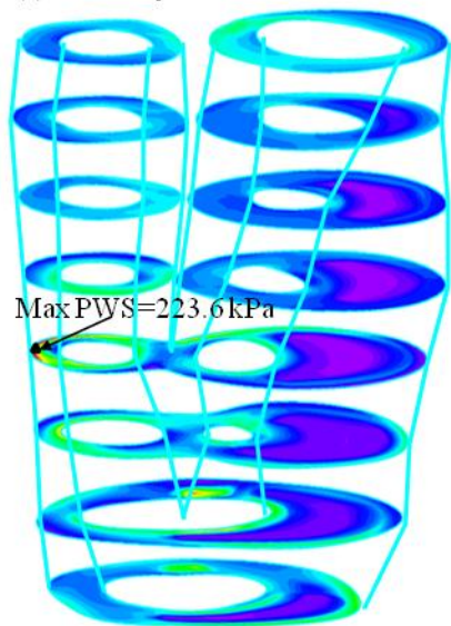
(a) Stress- P_1 , Stack View
