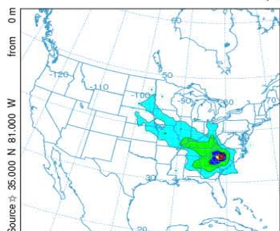
Spring (72 trajectories)
