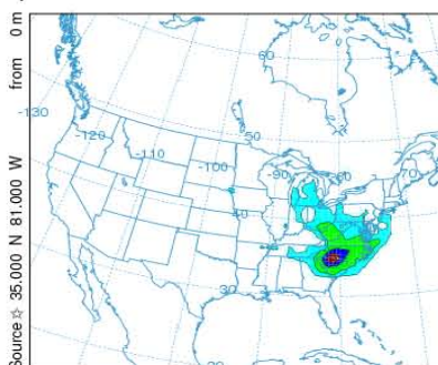
Summer (51 trajectories)
