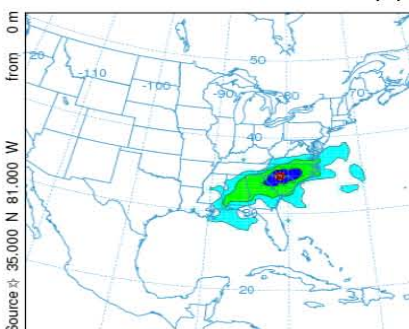
Spring (51 trajectories)
