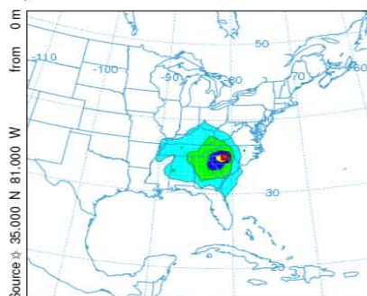
Summer (113 trajectories)
