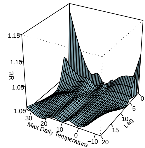
Without HW term, lag df=6, temp df = 8
