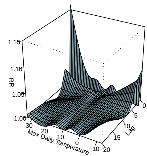
Without HW term, lag df=6, temp df = 6
