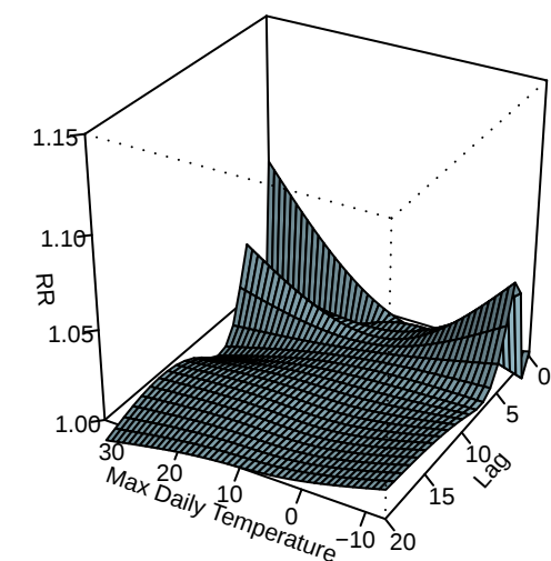
With HW indicator term, lag df=6, temp df = 3
