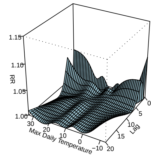
With HW indicator term, lag df=6, temp df = 8
