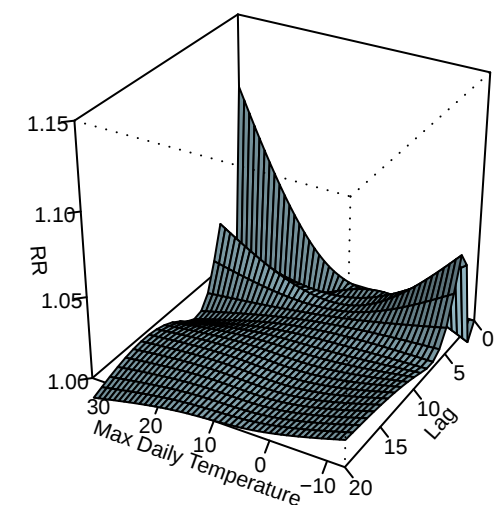
Without HW term, lag df=6, temp df = 3
