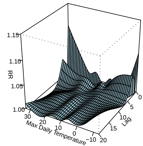
With HW duration term, lag df=6, temp df = 8
