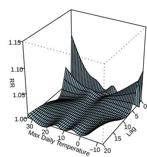
With HW indicator term, lag df=6, temp df = 6
