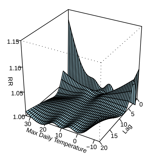
With HW duration term, lag df=6, temp df = 6
