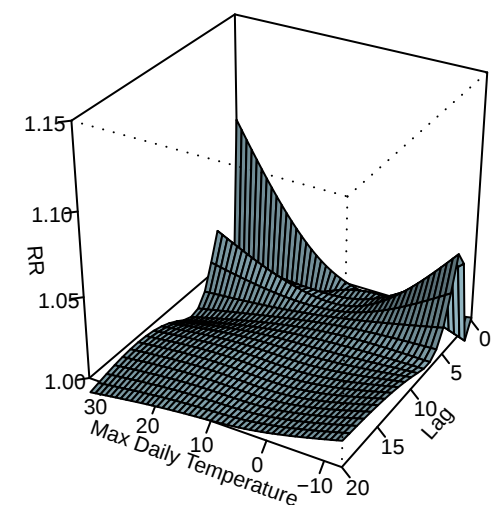
With HW duration term, lag df=6, temp df = 3
