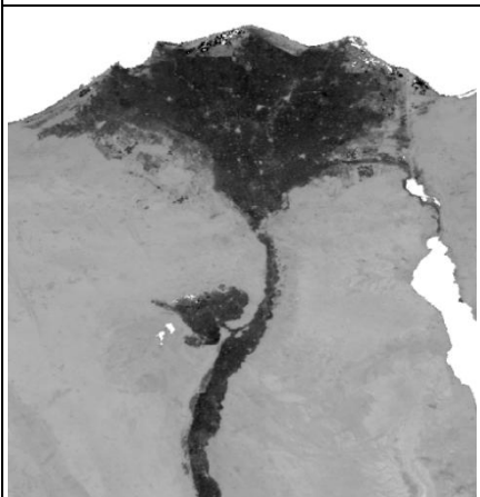
LSWI
