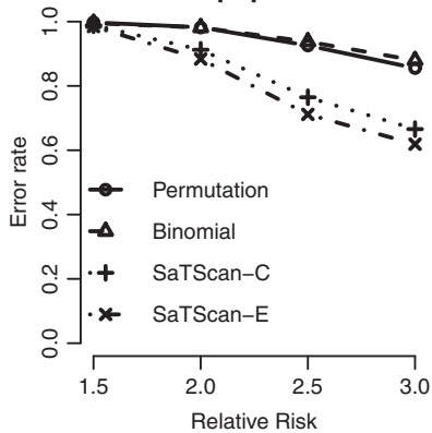
Error rate comparison of the Y-shaped cluster with fewer population size
