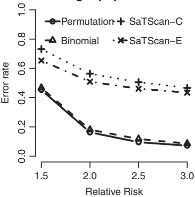
Error rate comparison of the circular cluster with larger population size
