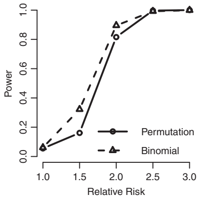
Powers with different RRs in detecting the long cluster
