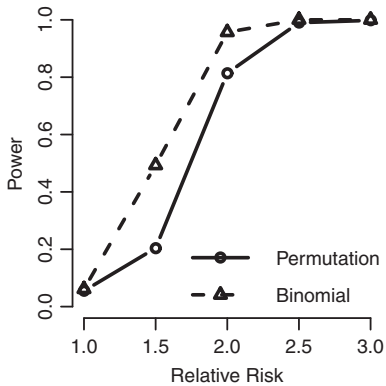
Powers with different RRs in detecting the Y-shaped cluster
