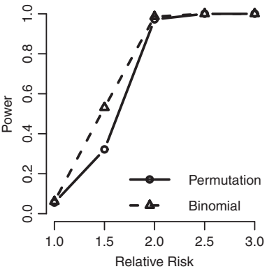
Powers with different RRs in detecting the circular cluster
