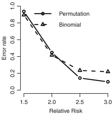
Error rates with different RRs in detecting the long cluster
