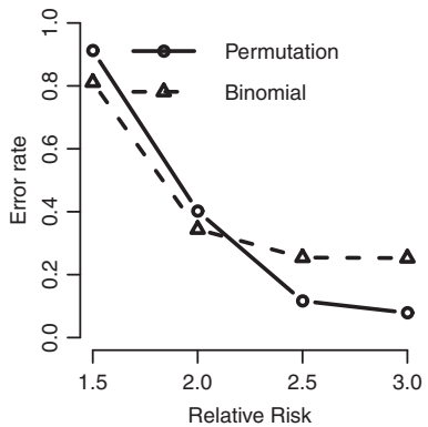
Error rates with different RRs in detecting the Y-shaped cluster
