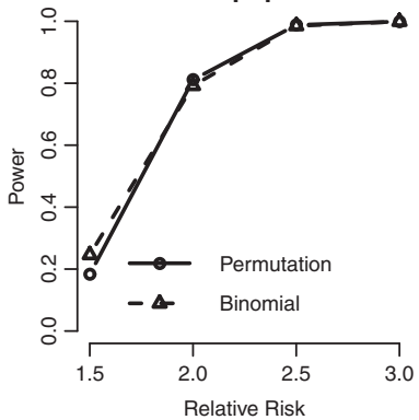
Powers with different RRs in detecting the long cluster with median population size
