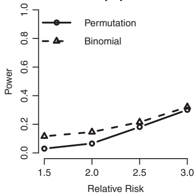
Powers with different RRs in detecting the Y-shaped cluster with fewer population size
