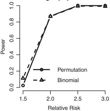
Powers with different RRs in detecting the circular cluster with larger population size
