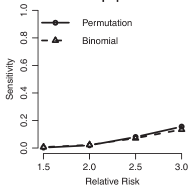
Sensitivities with different RRs in detecting the Y-shaped cluster with fewer population size
