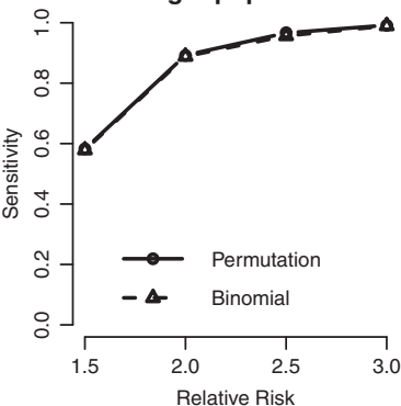
Sensitivities with different RRs in detecting the circular cluster with larger population size
