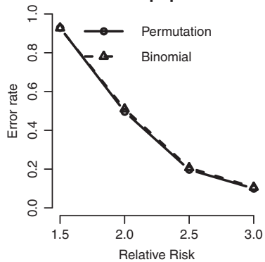
Error rates with different RRs in detecting the long cluster with median population size
