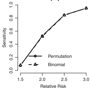
Sensitivities with different RRs in detecting the long cluster with median population size
