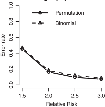
Error rates with different RRs in detecting the circular cluster with larger population size
