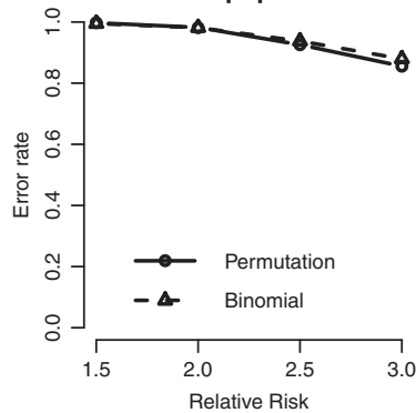
Error rates with different RRs in detecting the Y-shaped cluster with fewer population size
