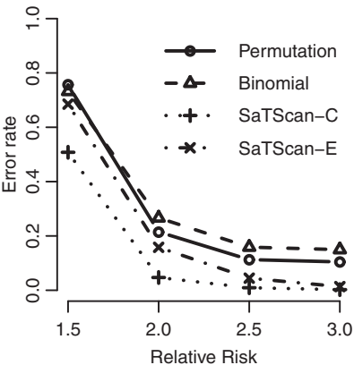
Error rate comparison of the circular cluster
