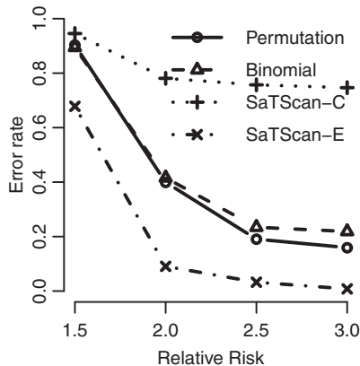
Error rate comparison of the long cluster
