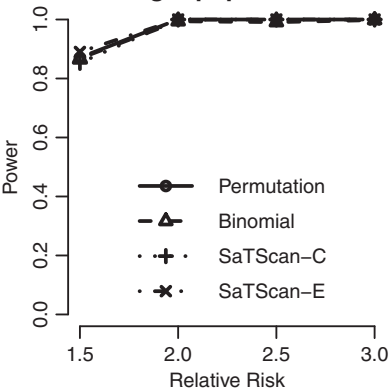
Power comparison of the circular cluster with larger population size
