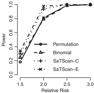
Power comparison of the long cluster with median population size
