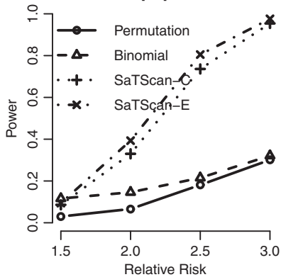
Power comparison of the Y-shaped cluster with fewer population size
