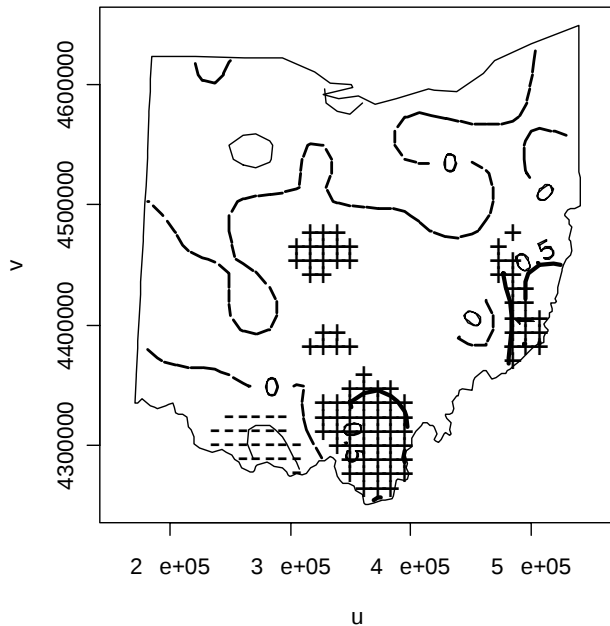
Log relative risk, bandwidth = 22647
