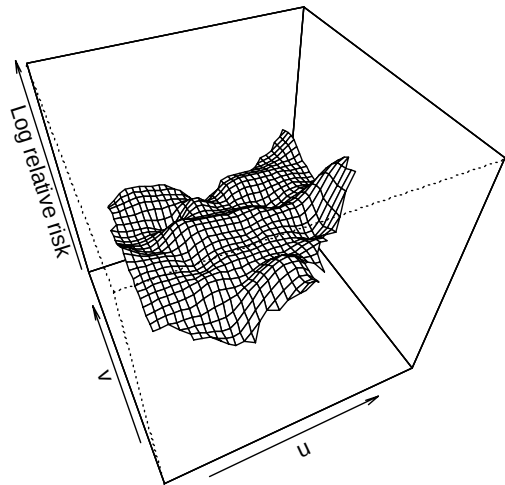
Log relative risk surface
