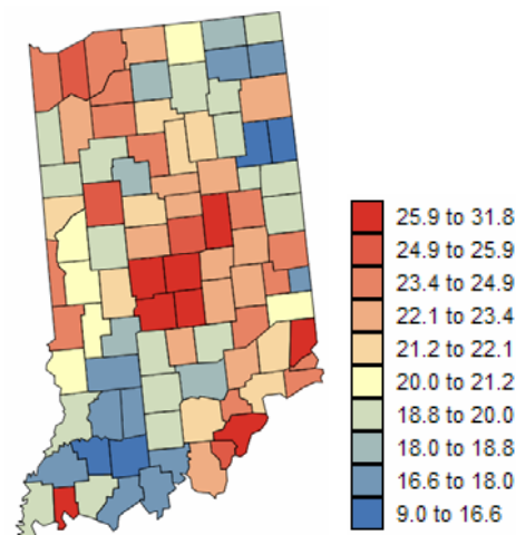
Bayesian estimates
