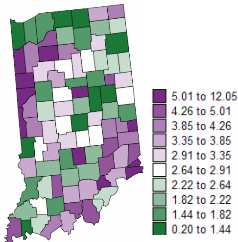
Bayesian variance
