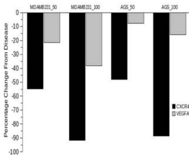
Effect of NFκB inhibition on CXCR4 and VEGFA
