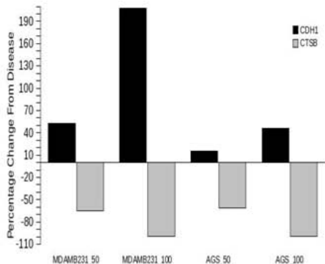
Effect of NFκB inhibition on CDH1 and CTSS
