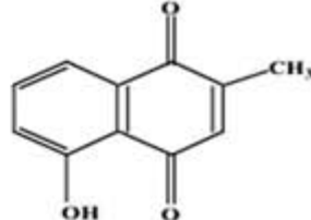
Plumbagin (5-hydroxy-2-methylnaphthalene-1,4-dione)
