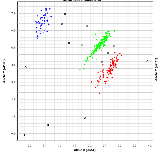
Allelic Discrimination Plot
