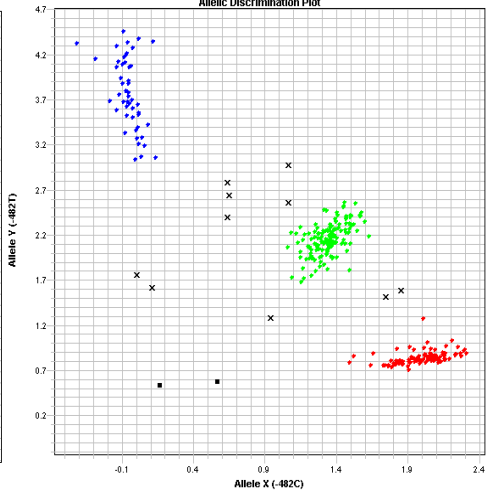
Allelic Discrimination Plot
