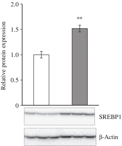
SREBP1
