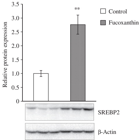
SREBP2
