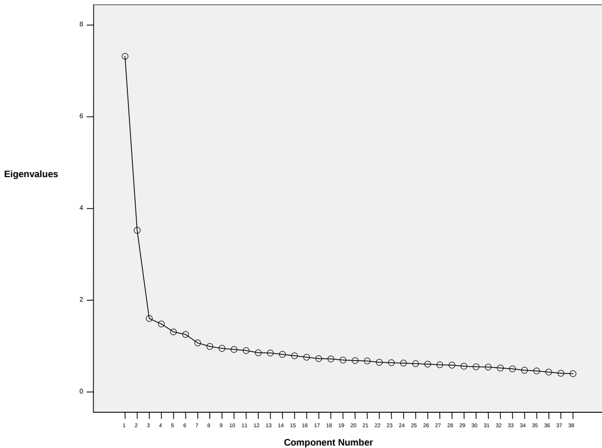
Scree-Plot for the International sample (n=5238)
