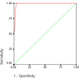
ROC Curve
