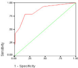
ROC Curve
