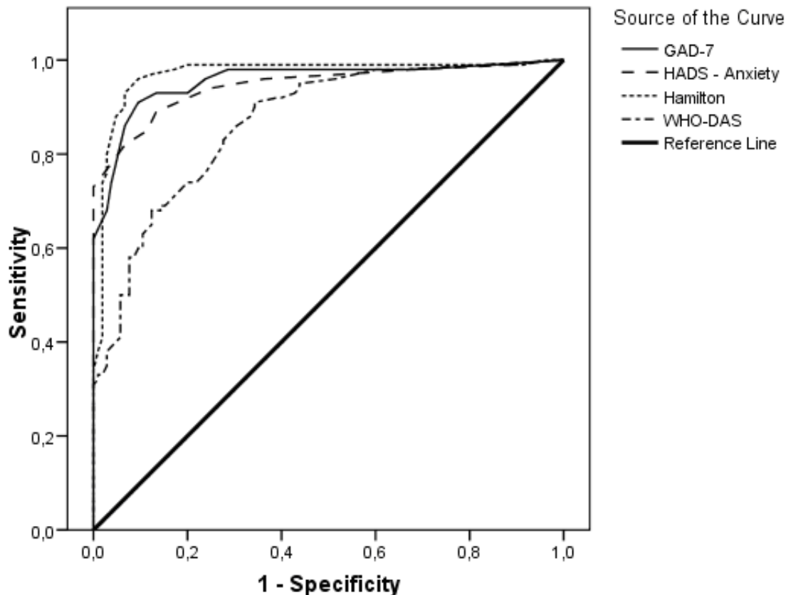
ROC Curve
