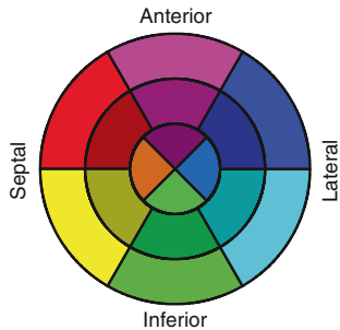
C: Standard Bullseye Segmentation of the Left Ventricle
