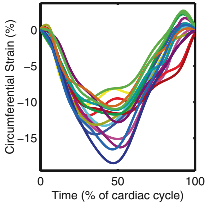
B: Example Strain Curves
