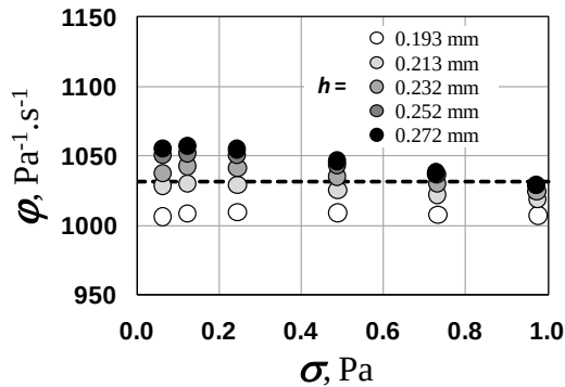
(a) \chi = 0
