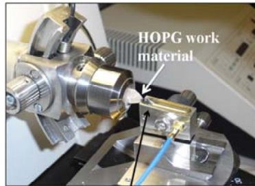
Ultra sharp wedge mounted on an ultrasonic oscillation system
