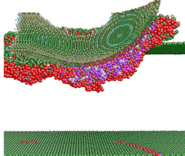
(c) Ge
