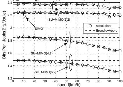
Energy Efficiency(distance:1km,BW:5MHz,(6,2,3))
