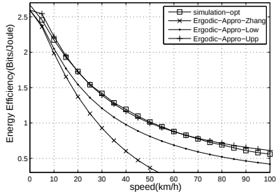
Energy Efficiency(distance:1km,BW:5MHz,(6,2,3))
