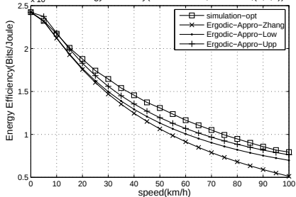
Energy Efficiency(distance:1km,BW:5MHz,(6,2,3))
