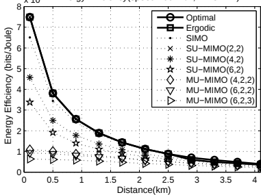
Energy Efficiency(speed:100km/h,BW:5MHz)
