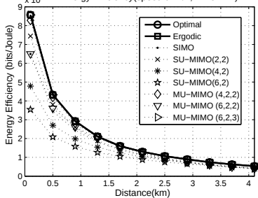
Energy Efficiency(speed:100km/h,BW:5MHz)
