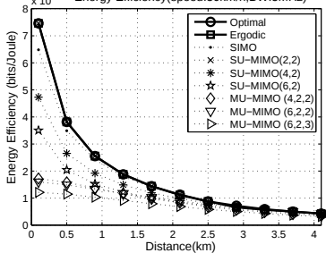
Energy Efficiency(speed:100km/h,BW:5MHz)
