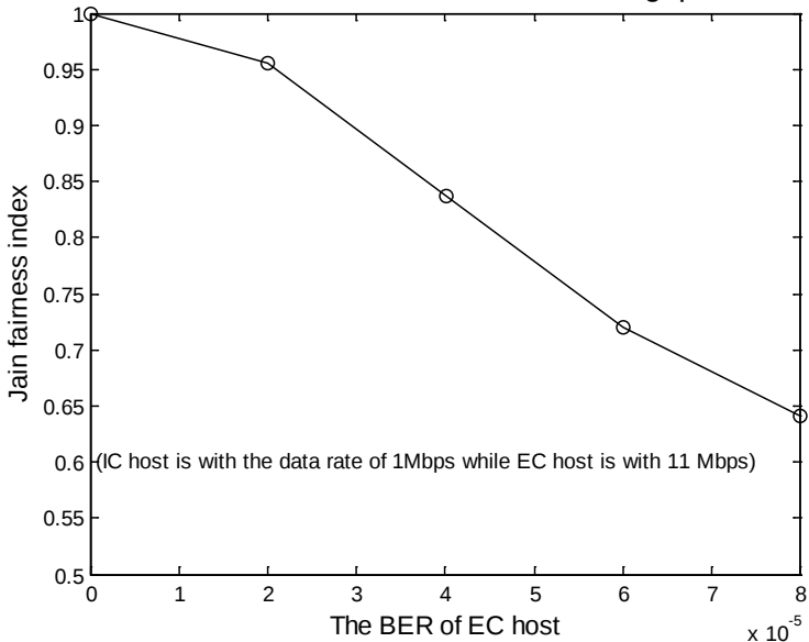
The fairness index in terms of throughput
