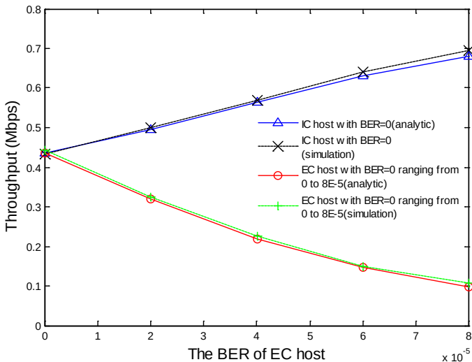
The throughput variations of two stations with diverse channel conditions
