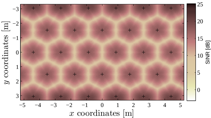
(b) Reuse partitioning ( K = 3 )
