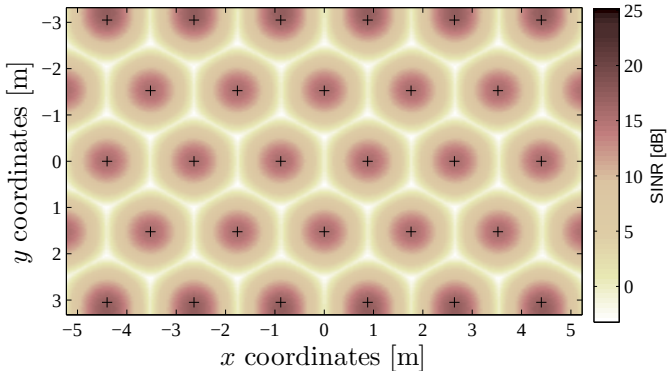
(a) Full reuse ( K = 1 )
