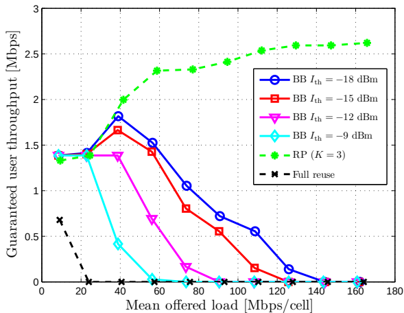
(a) Guaranteed user throughput
