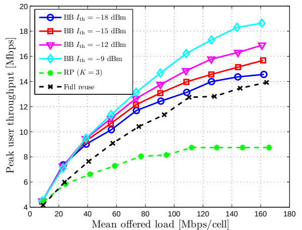
(b) Peak user throughput
