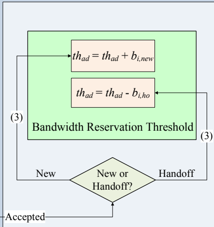
Adaptive Bandwidth Reservation (BR) Scheme
