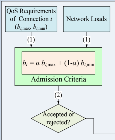
Dynamic Connection Admission Control (CAC) Algorithm
