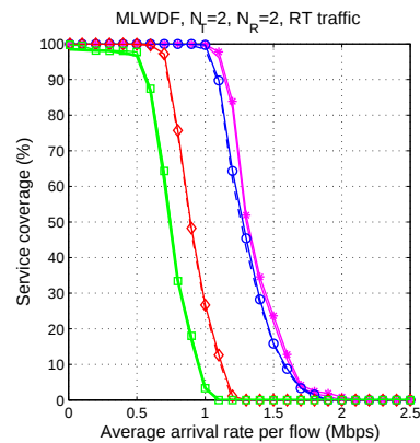
(e) Service coverage
