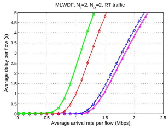
(b) Average delay per flow
