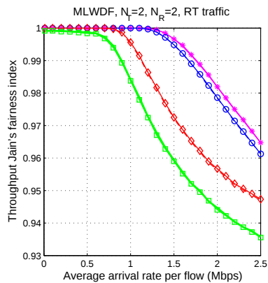
(c) Throughput Jain's fairness index
