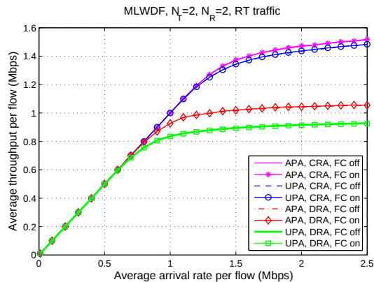
(a) Average throughput per flow
