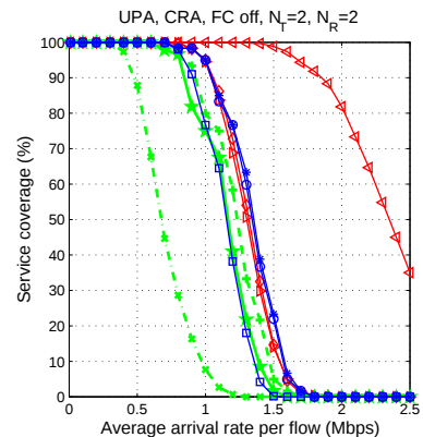
(e) Service coverage
