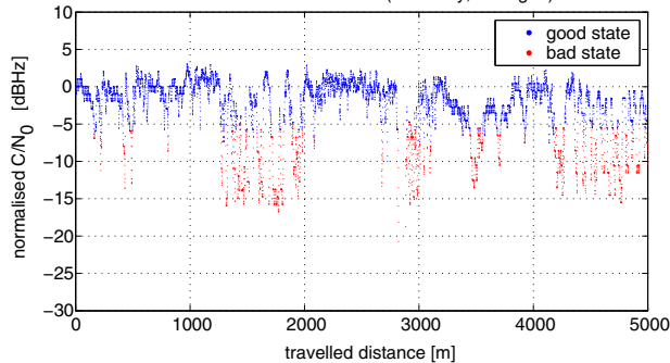
GNSS measurements (Germany, Erlangen)
