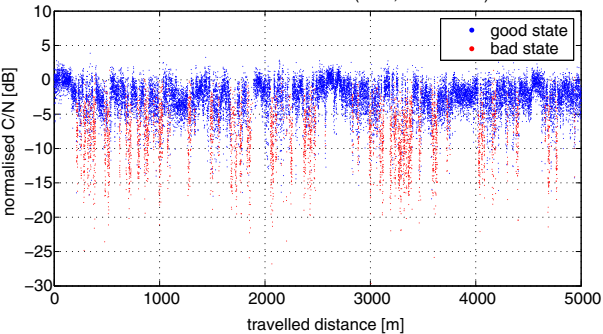
SDARS measurements (USA, East Coast)
