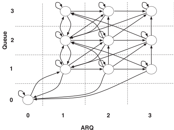
Combined ARQ-Queue
