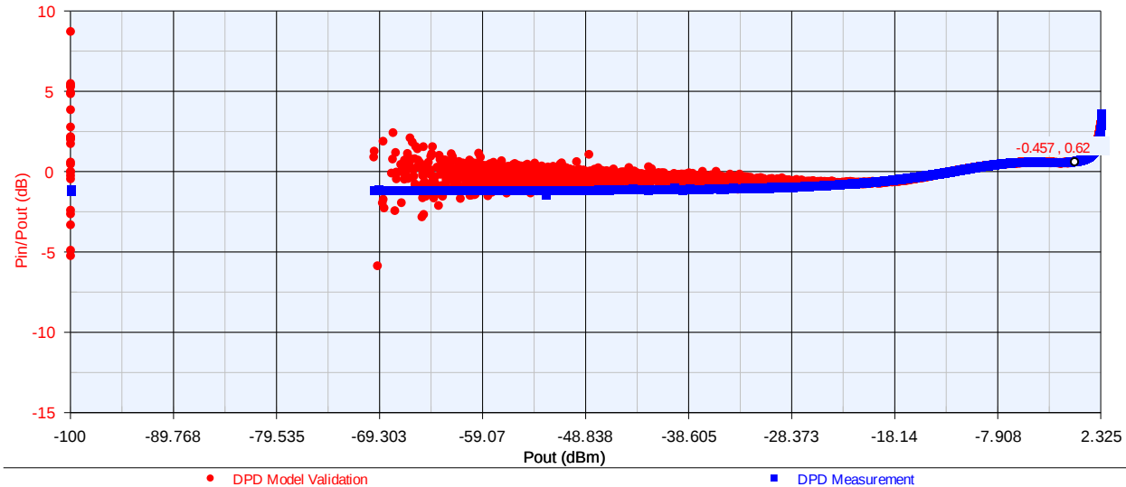
AM-AM Characteristic
