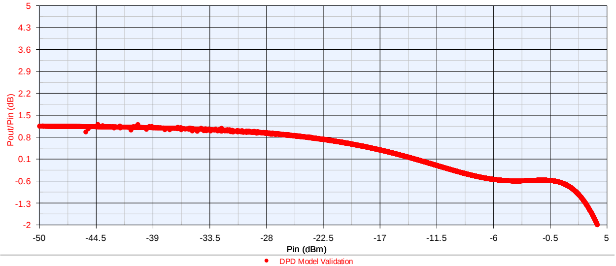
AM-AM Characteristic
