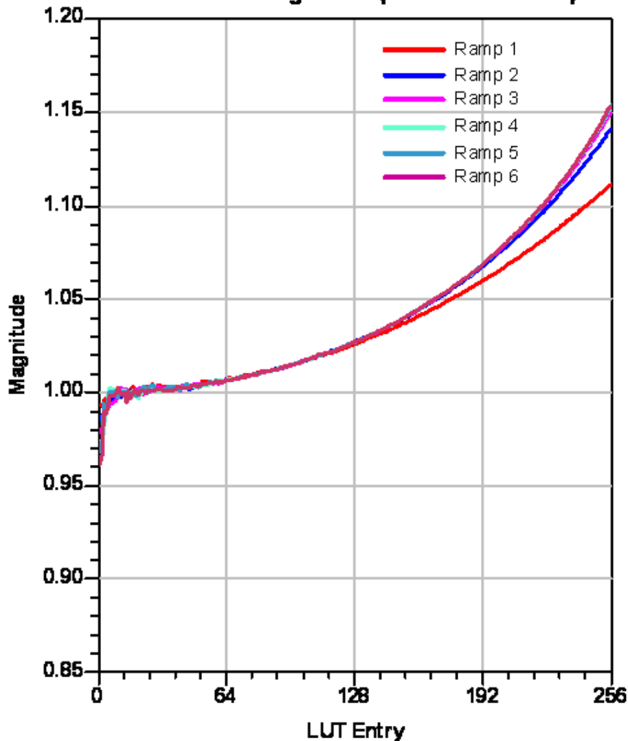
Coefficient Magnitude (iteration 1 thru 6)
