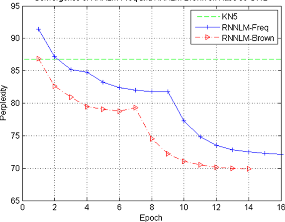
Convergence of RNNLM-Freq and RNNLM-Brown on Hub5'00-SWB
