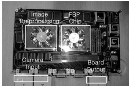
(b) Hardware board
