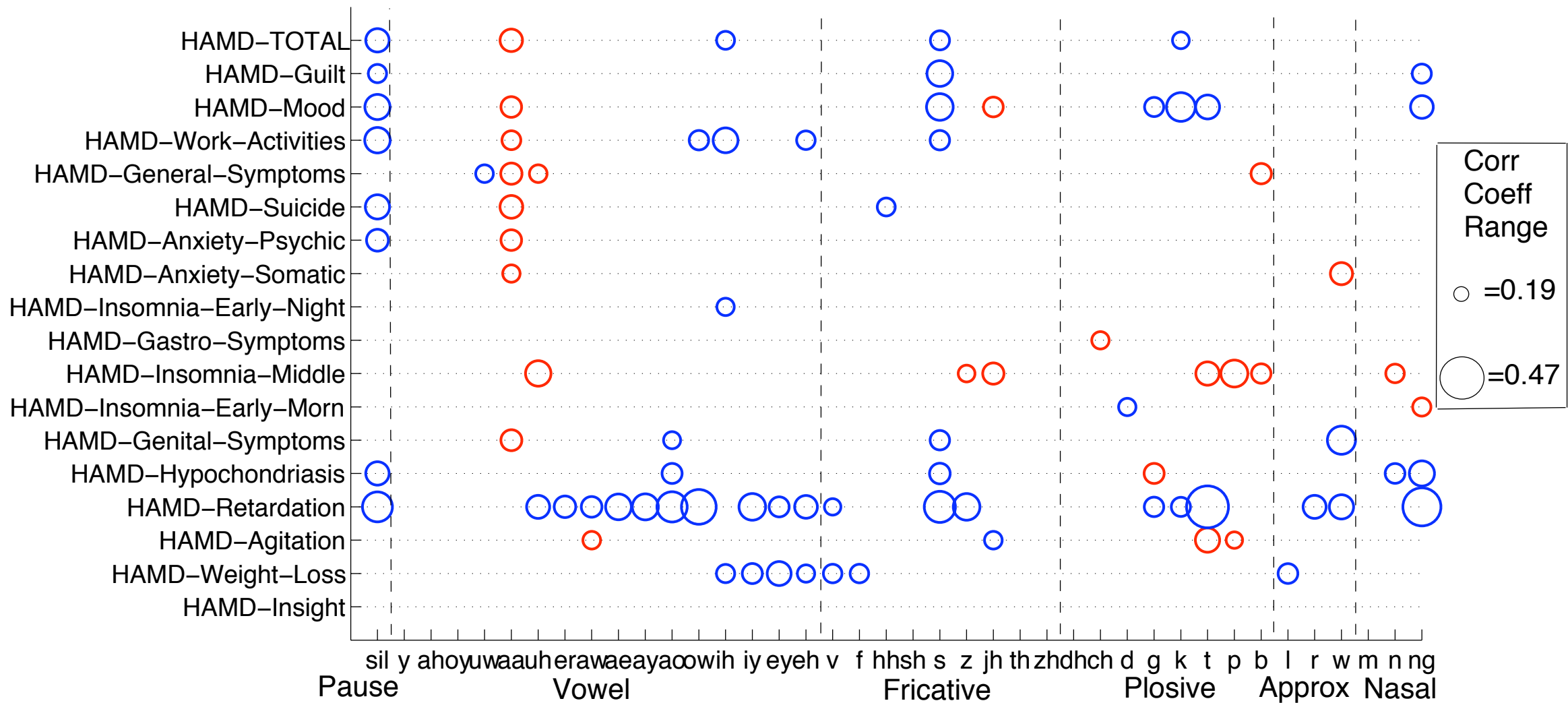
Correlation between Avg Phone Length and Score
